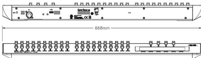
COLORSOURCE 40
