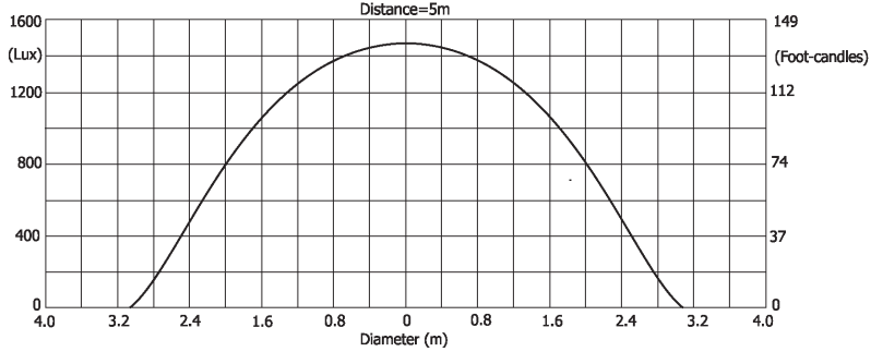
Illuminance distribution
